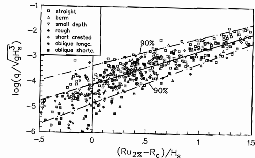
Figure 10 Overtopping formula and data
