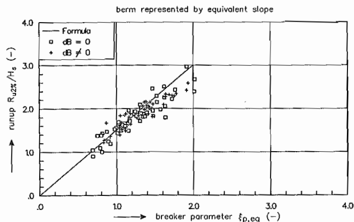
Figure 4 The influence of a berm on runup
