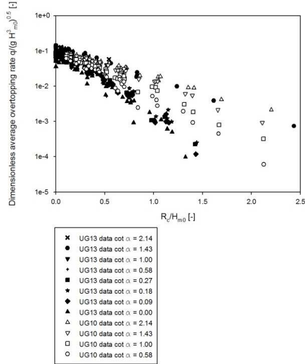
Figure 3. Dimensionless average overtopping rate q / (g H_{m0}^3)^{0.5} versus the relative freeboard R_C / H_{m0} for UG13 (black symbols) and UG10 data Victor (2012) (white symbols).
