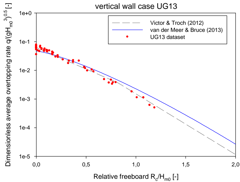
Figure 5. Dimensionless average overtopping rate q/(gH_{m0}^3)^{0.5} versus the relative freeboard R_c/H_{m0} for UG13 data compared to Victor & Troch (2012b) and van der Meer & Bruce (2013).
