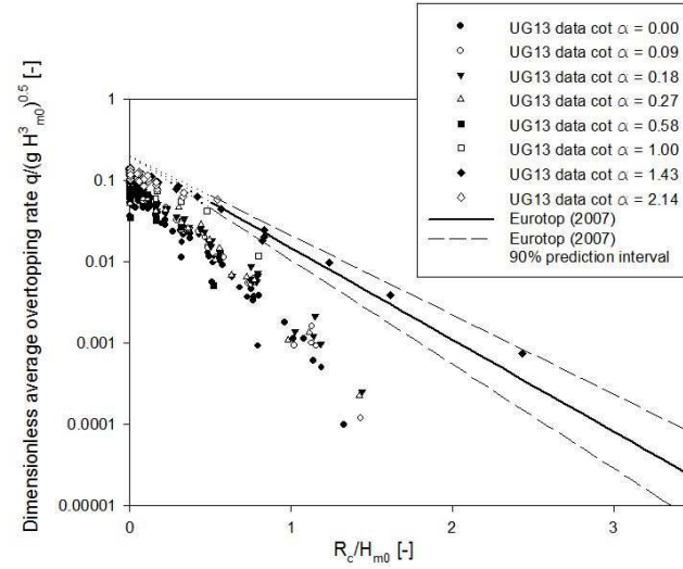
Figure 4. Dimensionless average overtopping rate q/(gH_{m0}^3)^{0.5} versus the relative freeboard R_c/H_{m0} for UG13 compared to the Eurotop (2007) overtopping prediction formula
