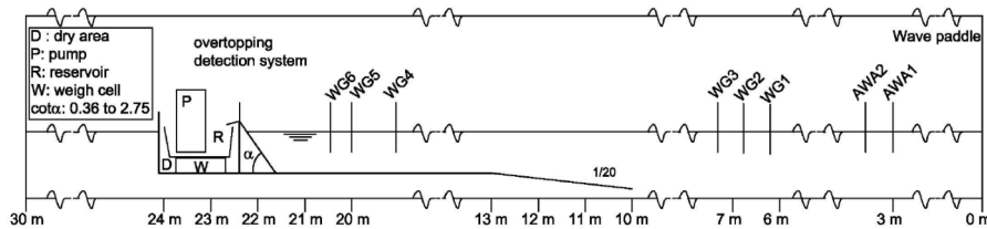
Figure 1. Cross section of the experimental test set-up, as used in Victor (2012).
