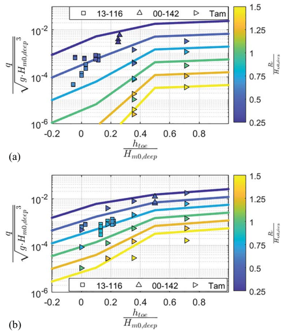
Fig. 10. Variation in relative discharge, q/\sqrt{g \cdot H_{m0,deep}^3} , with relative water depth ( h_{toe}/H_{m0,deep} ) and relative freeboard ( R_c/H_{m0,deep} ) for sloping structures (Table 2) with wave steepness ( s_{om-1,0} ): (a) 0.041; and (b) 0.018, for foreshore slopes ( \cot(m) ) = 30 and 35 and structure slope ( \cot(\alpha) ) = 3. Solid lines represent Eqs. (29)–(35) with \cot(m) = 32.5 .
