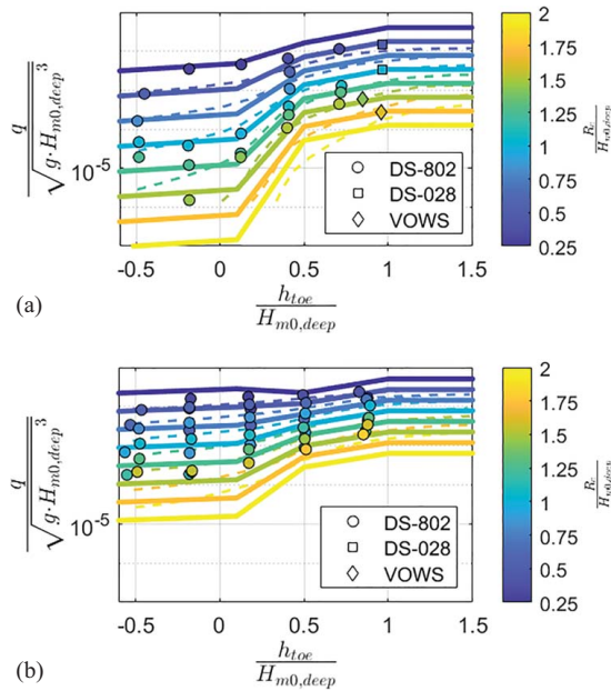
Fig. 7. Variation in relative discharge, q/\sqrt{g \cdot H_{m0,deep}^3} , with relative water depth ( h_{toe}/H_{m0,deep} ) and relative freeboard ( R_c/H_{m0,deep} ) for vertical structures (Table 3) with wave steepness ( s_{om-1,0} ): (a) 0.044; and (b) 0.015 for a foreshore slope ( \cot(m) ) = 10. The solid lines represent Eqs. (21)–(28), whereas the dashed lines represent the digitized design curves of Goda et al. (1975).
