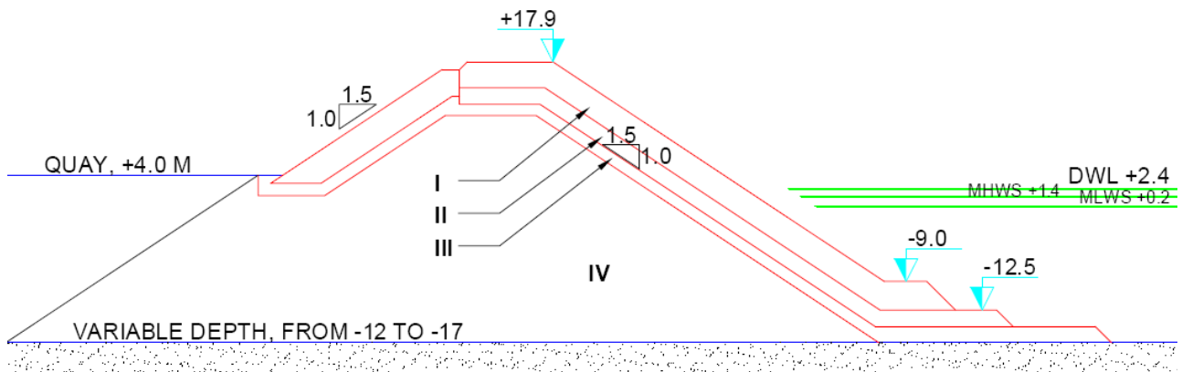
Figure 2. Icelandic-type Berm Breakwater cross section design for Húsavík
