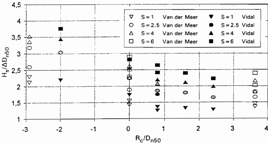
Figure 2. Stability at the front for fixed damage levels S
