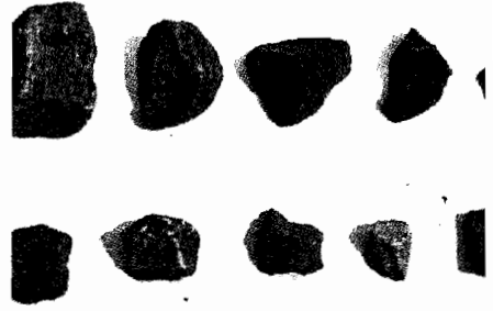
Type 2. Angular; D_{85} / D_{15} = 1.75 L/D > 2: 20\% L/D > 3: 0\%
