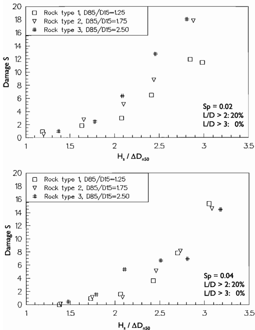
Figure 14. Influence of grading on stability
