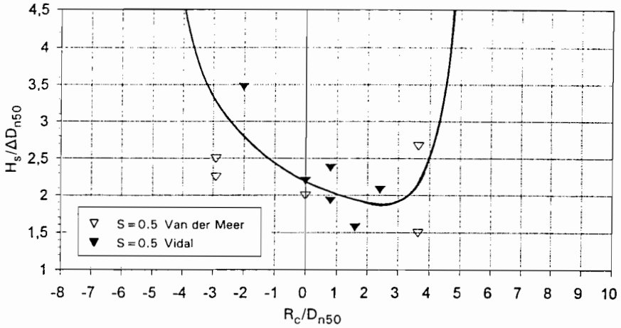
Figure 5. Stability rear for start of damage
