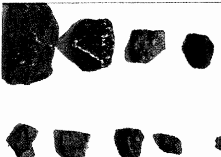
Type 3. Angular; D_{85} / D_{15} = 2.50 L/D > 2: 20\% L/D > 3: 0\%
