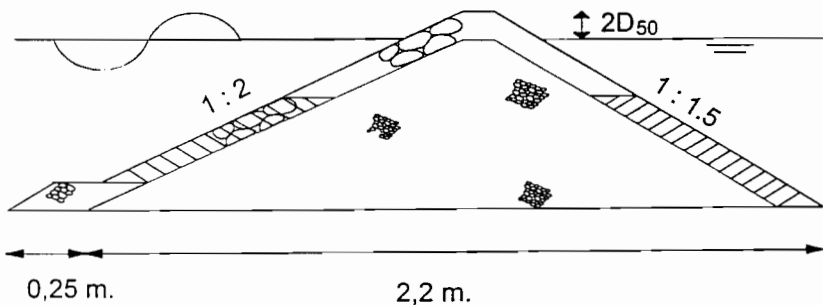
Figure 11. Tested cross-section
