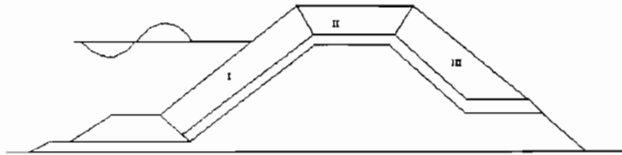
Figure 1. Division of armour layer in three segments
