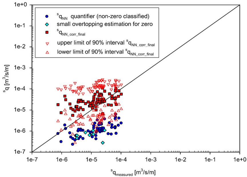
Fig. 10. Combined classifier–quantifier prediction of Ostia measurements.
