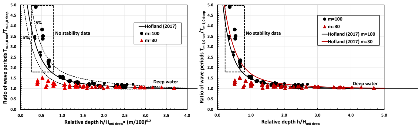
Figure 8: The change in spectral wave period over shallow foreshores according to Hofland et al. (2017,) but now with the present data on foreshore slopes with m=100 and 30. Left: with the influence of foreshore slope according to Hofland et al. (2017 – Equation 4) included in the x-axis. Right: without influence of the foreshore in the x-axis.
