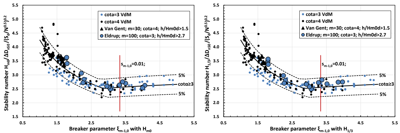
Figure 12: Stability for an impermeable structure and slope angles 1:3 and 1:4 on foreshore slopes with m=30 and 100, outside depth limited wave conditions with h/H_{m0\text{ deep}} > 1.5 . Solid black line is described by Eqs. 1-3. Left graph with the spectral wave height H_{m0} , right graph with the significant wave height H_{1/3} .
