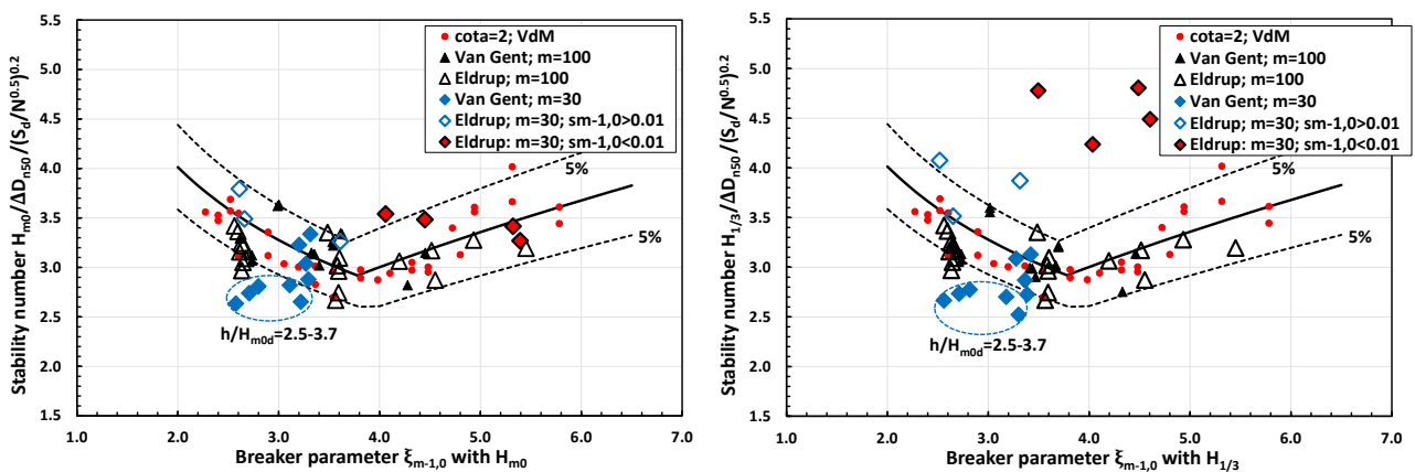
Figure 11: Stability for a permeable structure and slope angle 1:2 on foreshore slopes with m=30 and 100, and outside depth limited wave conditions with h/H_{m0 \text{ deep}} > 1.5 . Solid black line is described by Eqs. 1-3. Left graph with the spectral wave height H_{m0} . Right graph with the significant wave height H_{1/3} , showing a significant deviation for the nonlinear shoaling waves with very low wave steepness (red diamonds in the graphs).
