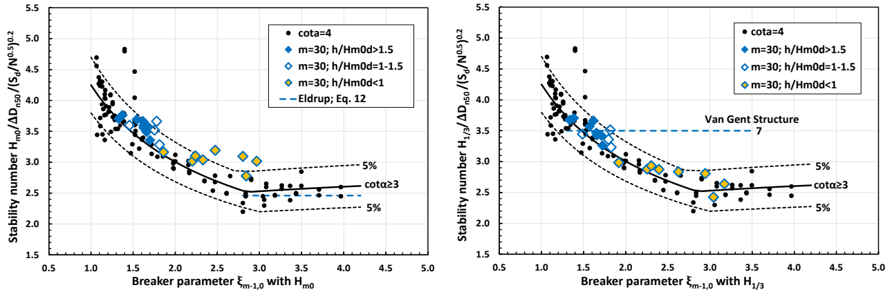
Figure 16: Stability for an impermeable core ( P=0.1 ) and \cot\alpha = 4 in shallow and very shallow water. The solid line gives the rewritten Van der Meer formula (Equations 1-3), the horizontal line in the left graph gives Equation 12 of Eldrup and Lykke Andersen (2019a) and the line in the right graph gives Equation 11, the simplified formula by Van Gent et al. (2003). Left graph with the spectral wave height, H_{m0} , right graph with the significant wave height, H_{1/3} .
